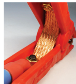
Braided copper bonding strap sends continuous current to both jaws for better amperage
