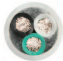
10 AWG ROUND
